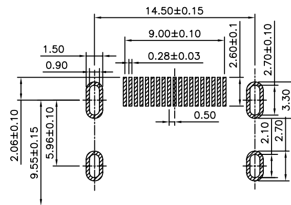
Recommended PCB Layout T=1.6±0.15
