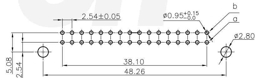
PCB Layout
